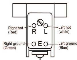
Terminals
